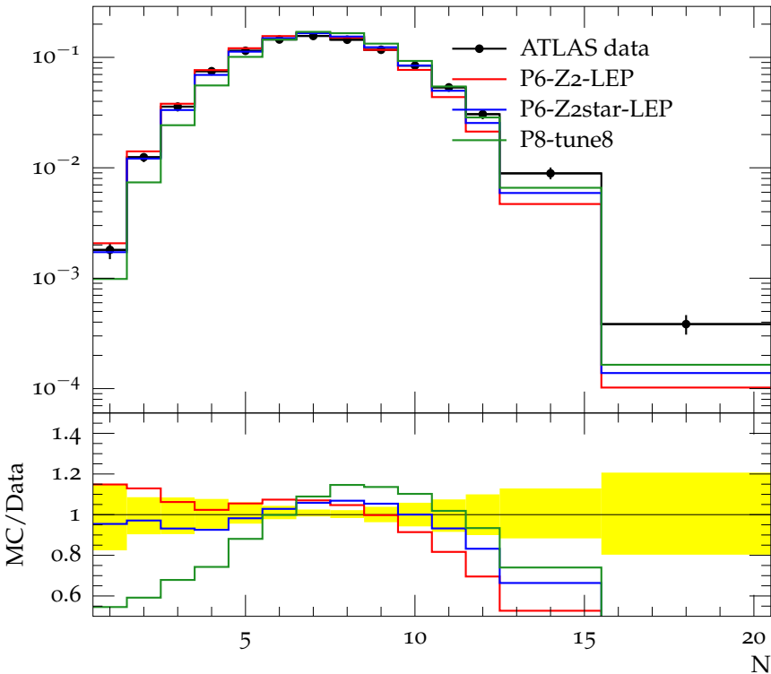
Charged jet multiplicity (anti- k_t , R = 0.6 , y 0.0-1.9, p_\perp 10.0-15.0)
