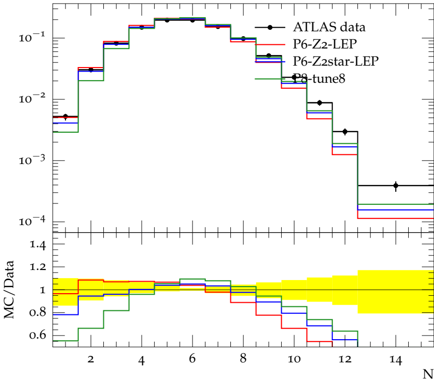
Charged jet multiplicity (anti- k_t , R = 0.6 , y 0.0-1.9, p_\perp 6.0-10.0)
