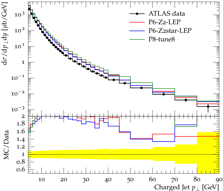
Charged jet cross section vs. p_{\perp} (anti- k_t , R = 0.6 , y 1.5-1.9)
