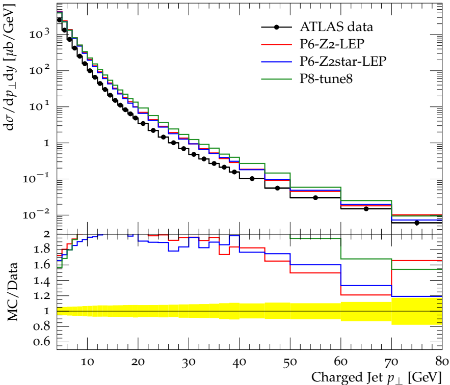
Charged jet cross section vs. p_{\perp} (anti- k_t , R = 0.6 , y 0.5-1.0)
