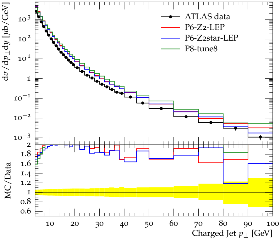
Charged jet cross section vs. p_{\perp} (anti- k_t , R = 0.6, y 0.0-0.5)
