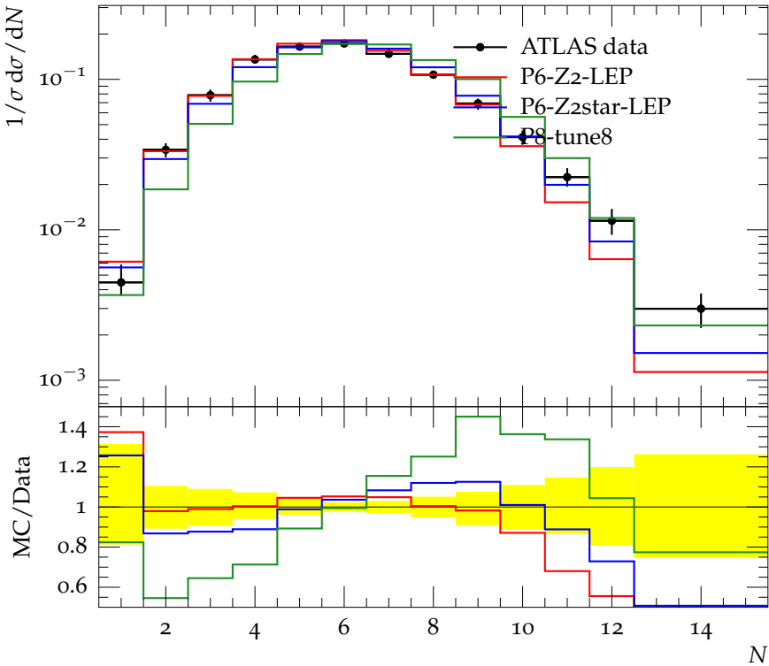
Charged jet multiplicity (anti- k_t , R = 0.4 , y 1.5-1.9, p_\perp 15.0-24.0)
