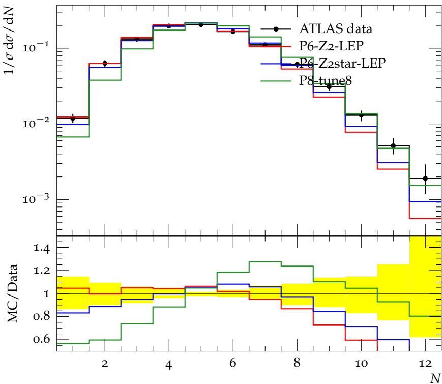
Charged jet multiplicity (anti- k_t , R = 0.4 , y 1.5-1.9, p_\perp 10.0-15.0)
