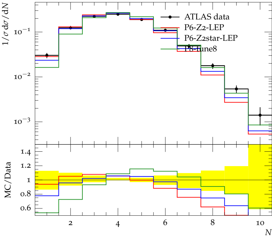
Charged jet multiplicity (anti- k_t , R = 0.4 , y 1.5-1.9, p_\perp 6.0-10.0)
