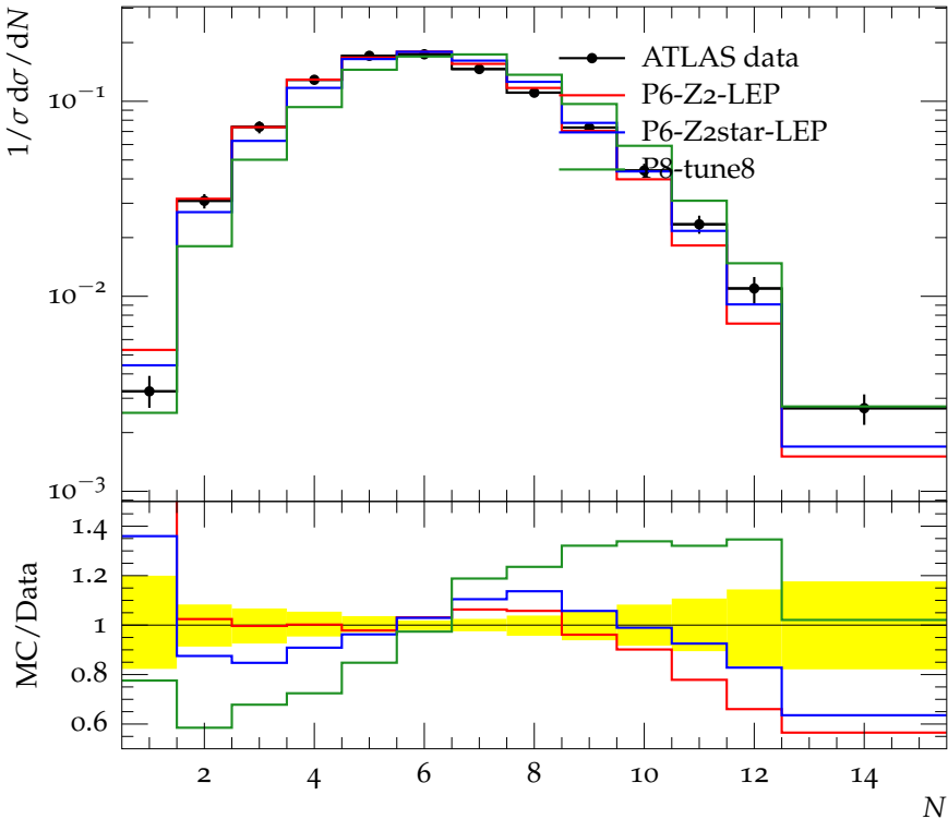
Charged jet multiplicity (anti- k_t , R = 0.4 , y 1.0-1.5, p_\perp 15.0-24.0)
