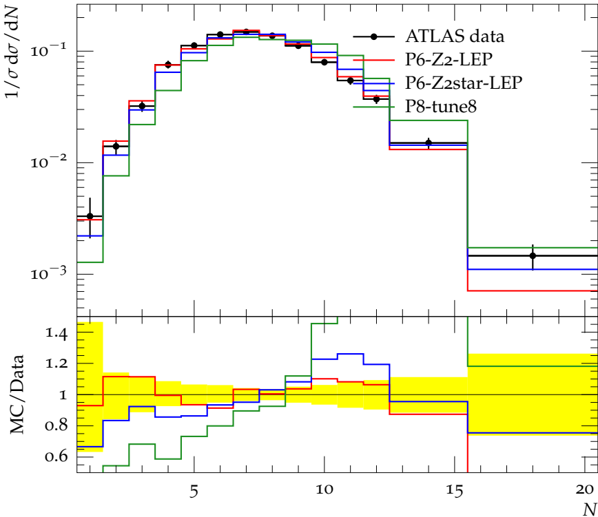
Charged jet multiplicity (anti- k_t , R = 0.4 , y 0.5-1.0, p_\perp 24.0-40.0)
