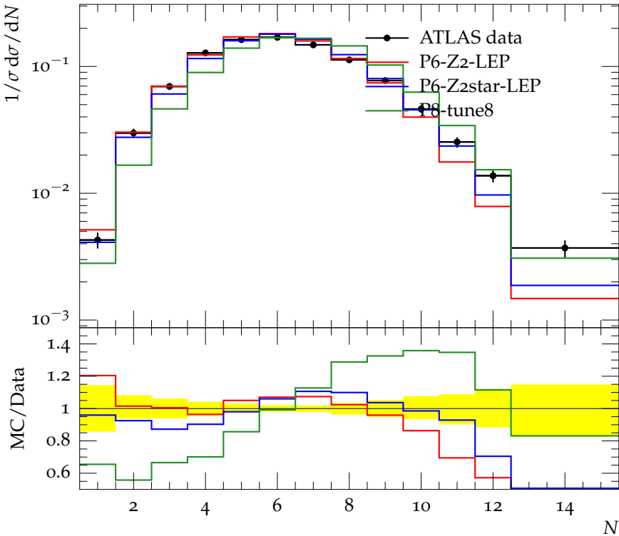
Charged jet multiplicity (anti- k_t , R = 0.4 , y 0.5-1.0, p_\perp 15.0-24.0)
