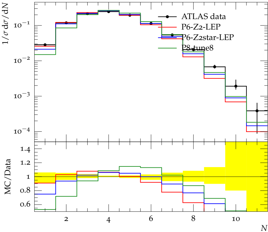
Charged jet multiplicity (anti- k_t , R = 0.4 , y 0.5-1.0, p_\perp 6.0-10.0)
