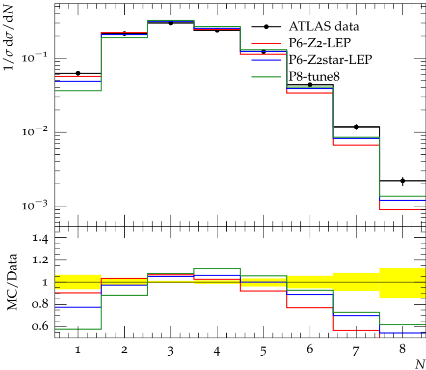
Charged jet multiplicity (anti- k_t , R = 0.4 , y 0.5-1.0, p_\perp 4.0-6.0)
