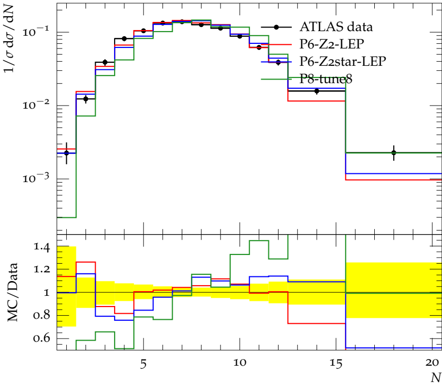
Charged jet multiplicity (anti- k_t , R = 0.4 , y 0.0-0.5, p_\perp 24.0-40.0)
