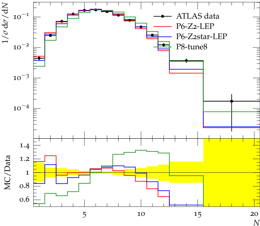
Charged jet multiplicity (anti- k_t , R = 0.4 , y 0.0-0.5, p_\perp 15.0-24.0)
