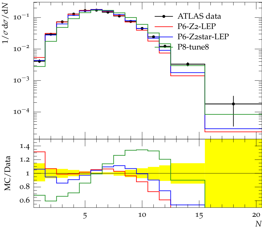
Charged jet multiplicity (anti- k_t , R = 0.4 , y 0.0-1.9, p_\perp 15.0-24.0)
