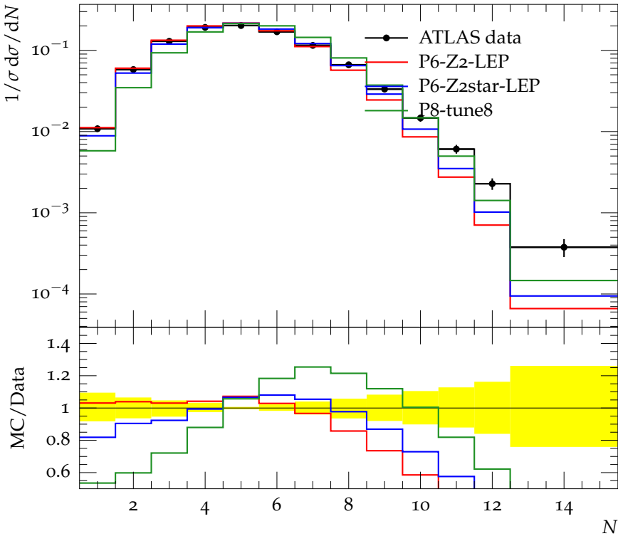
Charged jet multiplicity (anti- k_t , R = 0.4 , y 0.0-1.9, p_\perp 10.0-15.0)
