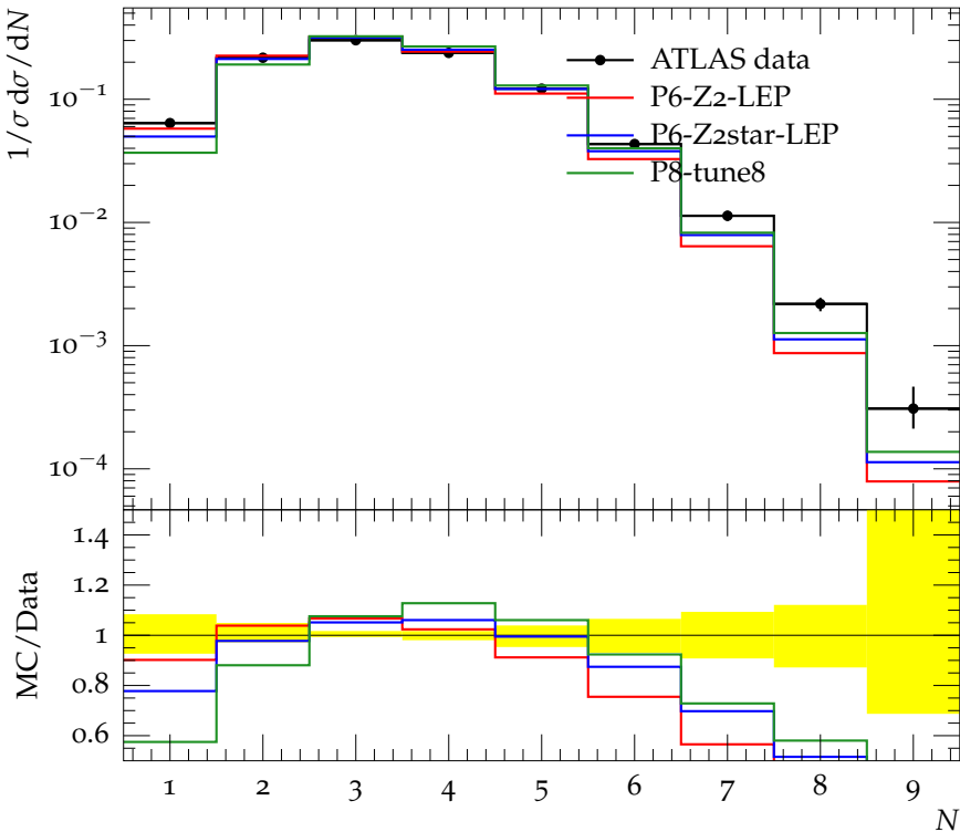
Charged jet multiplicity (anti- k_t , R = 0.4 , y 0.0-1.9, p_\perp 4.0-6.0)
