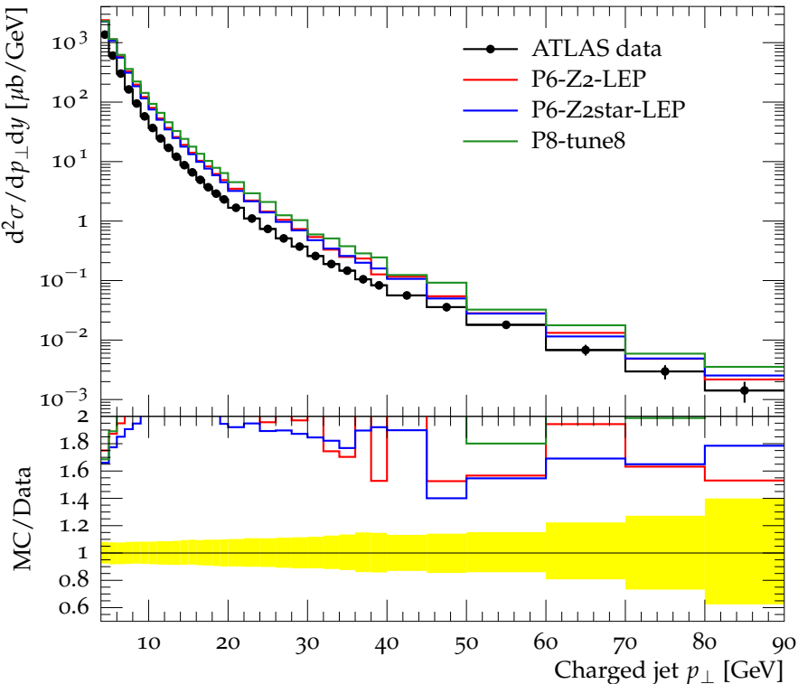
Charged jet cross section vs. p_{\perp} (anti- k_t , R = 0.4 , y 1.5-1.9)
