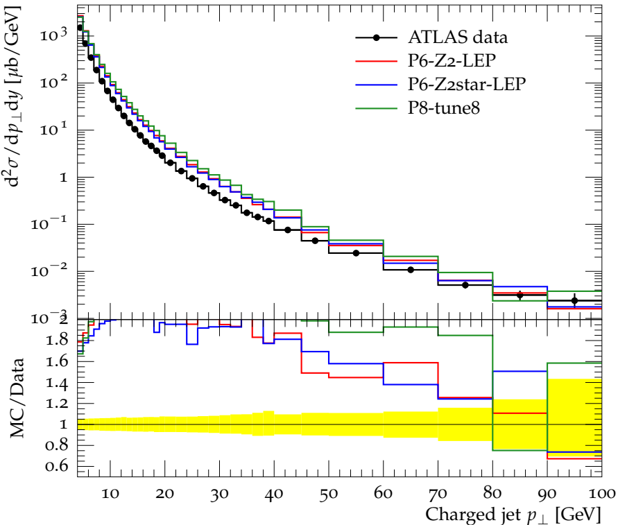
Charged jet cross section vs. p_{\perp} (anti- k_t , R = 0.4 , y 0.5-1.0)
