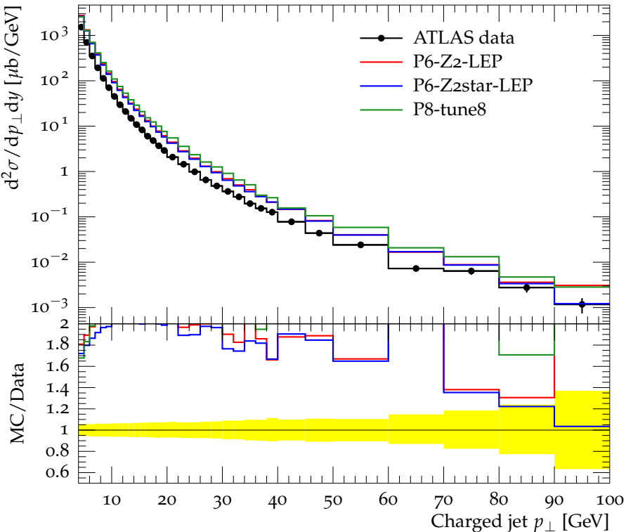
Charged jet cross section vs. p_{\perp} (anti- k_t , R = 0.4 , y 0.0-0.5)
