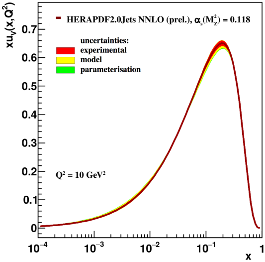
H1 and ZEUS preliminary
