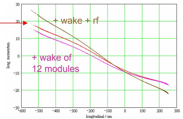
long. phase space @ 2.4 GeV before BC2
