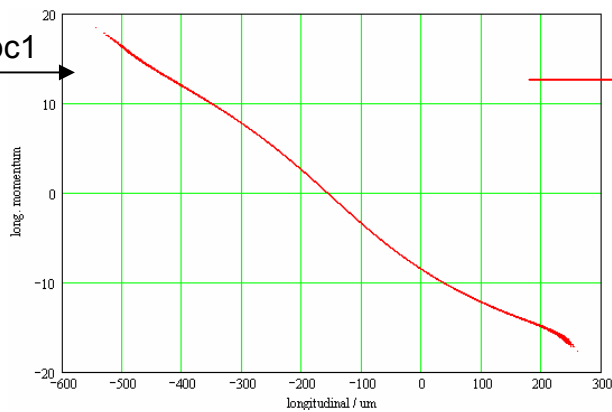
long. phase space @ 500 MeV after BC1
