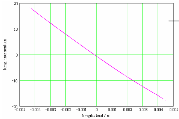
long. phase space @ 500 MeV before BC1
