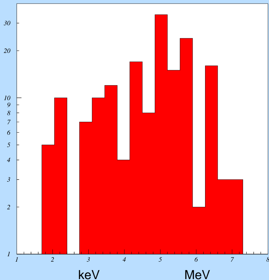
Energy spectrum
