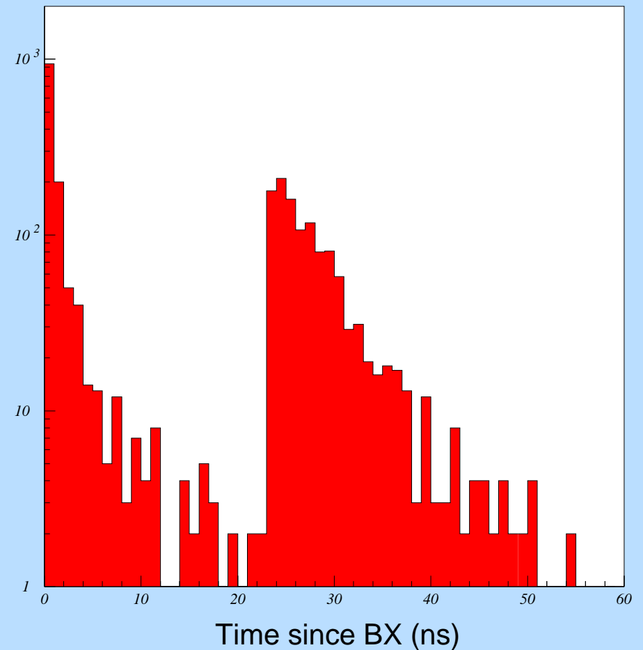
Time structure
