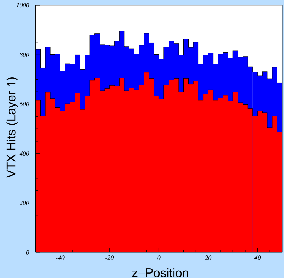
Longitudinal distribution
