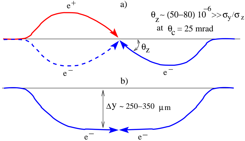
Figure 11: Trajectories of electrons (positrons) in the presence of the solenoid field and a crab-crossing angle. At the lower figure, the e^-e^- collision angle is made zero using shifted quads.
