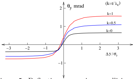
Figure 5: Deflection curves in \gamma\gamma collisions for various conversion efficiencies.
