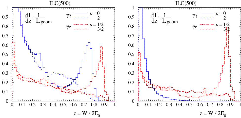
Figure 2: \gamma\gamma , \gamma e luminosity spectra, left: both beams are converted to photons; right: only one beam is converted to photons. See parameters in the text. \gamma\gamma .
