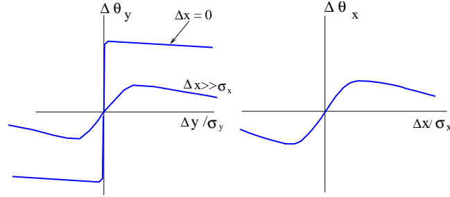
Figure 3: Typical beam-beam deflection in e^+e^- and \gamma\gamma collisions
