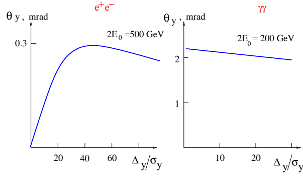
Figure 3: Typical beam-beam deflection in e^+e^- and \gamma\gamma collisions
