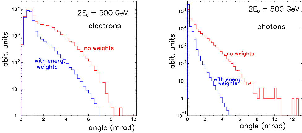
Figure 13: Angular distributions of electrons (left) and photons (right) after the conversion and interaction points.
