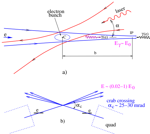
Figure 1: Scheme of \gamma\gamma, \gamma e collider
