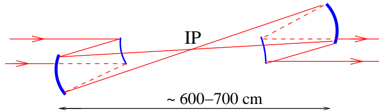
Figure 18: Laser optics inside the detector (alternative scheme).
