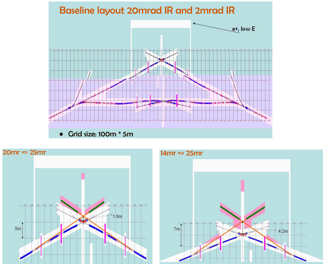
Figure 16: Layout of the interaction regions at the ILC. The bottom figures show the upgrade path from e^+e^- to \gamma\gamma according to [29]. See the author's alternative suggestion in the text below.
