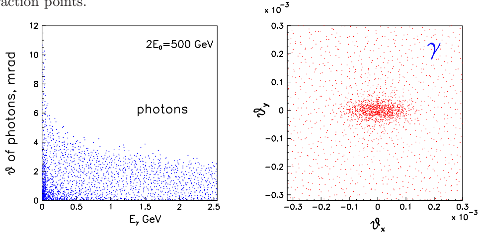
Figure 14: Energy-angular distributions of beamstrahlung photons (left) and the angular distribution of Compton photons (right).
