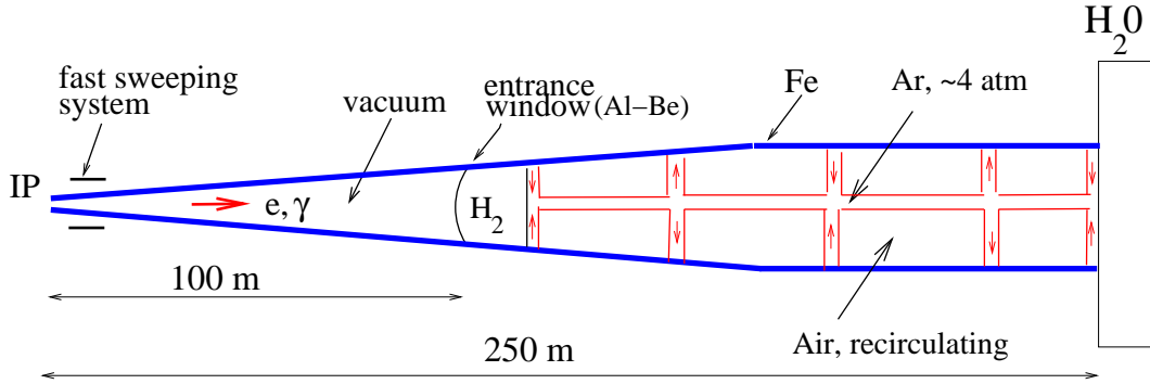
Figure 15: An idea for the photon collider beam dump.
