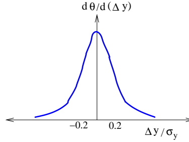
Figure 6: Derivative of the typical deflection curve
