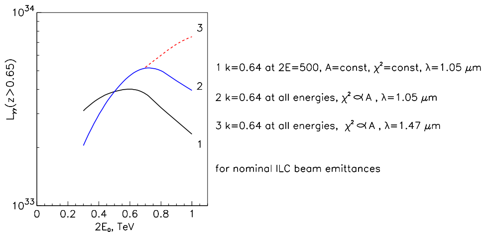
Figure 19: Dependence of the \gamma\gamma luminosity on the energy.
