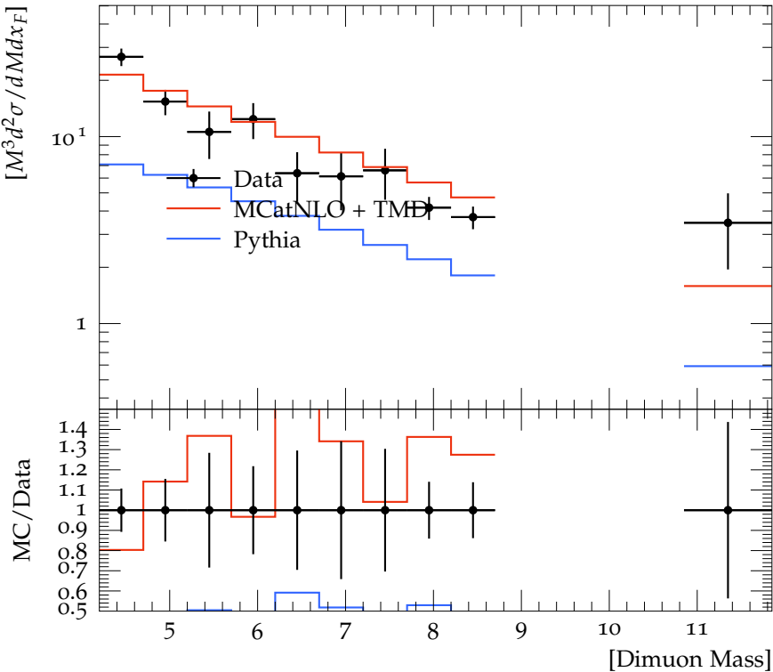
[Dimuon mass vs Invariant form for H cross section]
