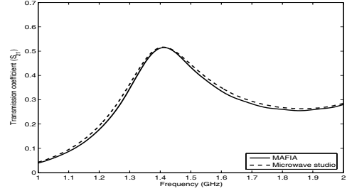
Figure 4: Amplitude of the transmission coefficient ( s_{21} ) from port 1 to port 2 versus frequency.
