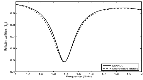
Figure 3: Amplitude of the reflection coefficient ( S_{11} ) at port 1 versus frequency.
