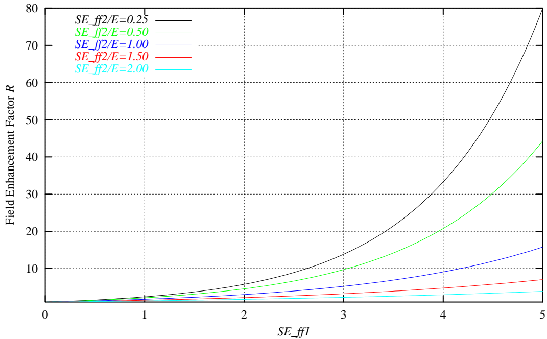
Fig. 3 Field Enhancement Factor R as function of parameter SE\_ff1 for various ratios of SE\_ff2 to the applied gradient E .
