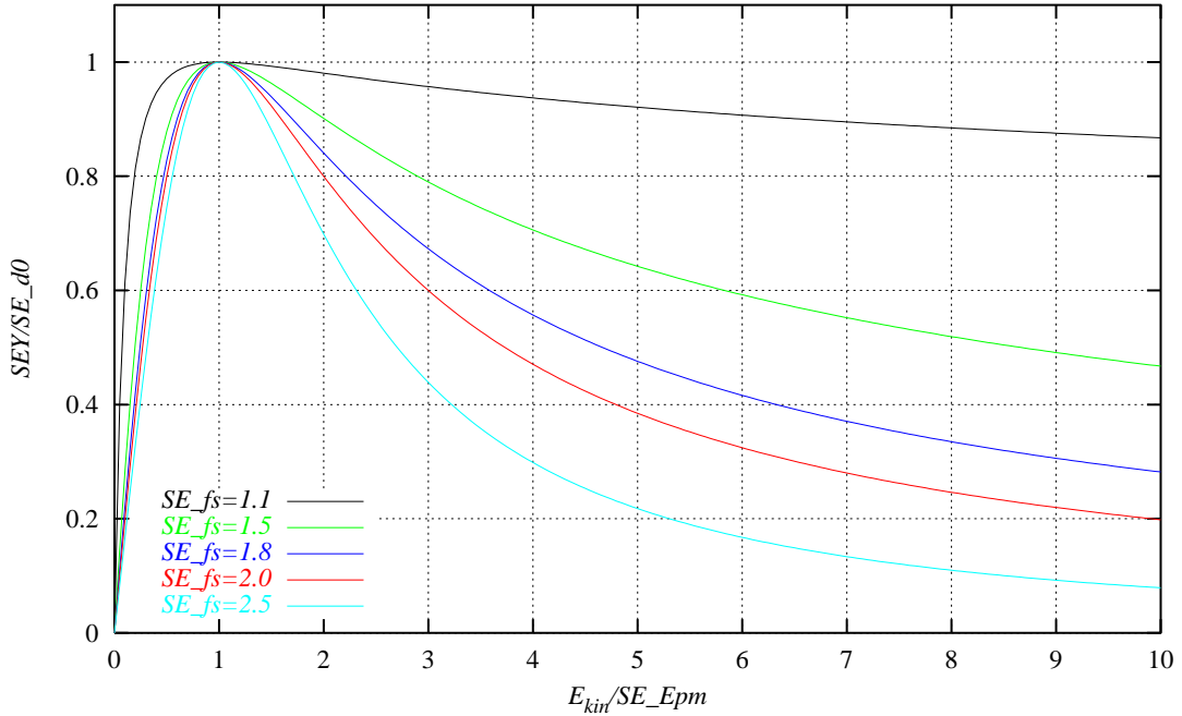
Fig. 2 Secondary Electron Yield for various parameters SE_{fs} .
