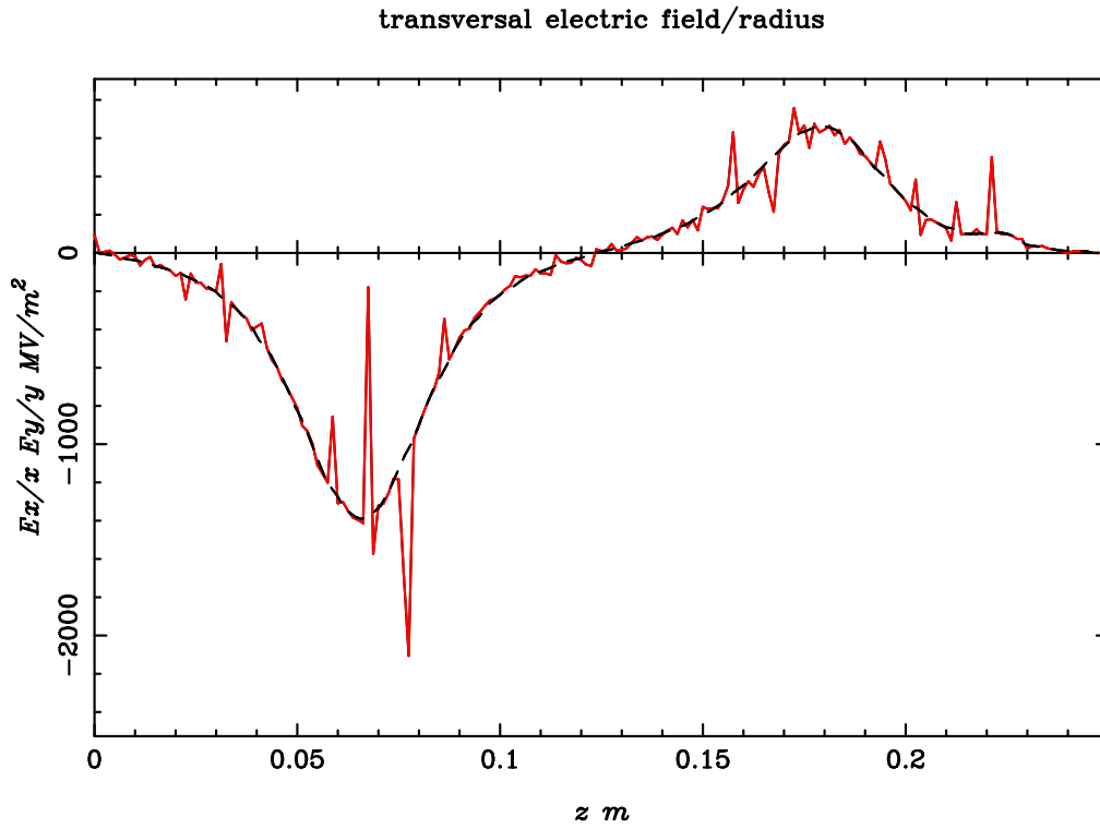
Fig. 5 Example of the transverse electric field components calculated with the field expansion formulas from an inaccurate field table. The numerical noise in the original data (red, solid line) is removed by the smoothing procedure (dashed, black line) without influence onto the average behavior.
