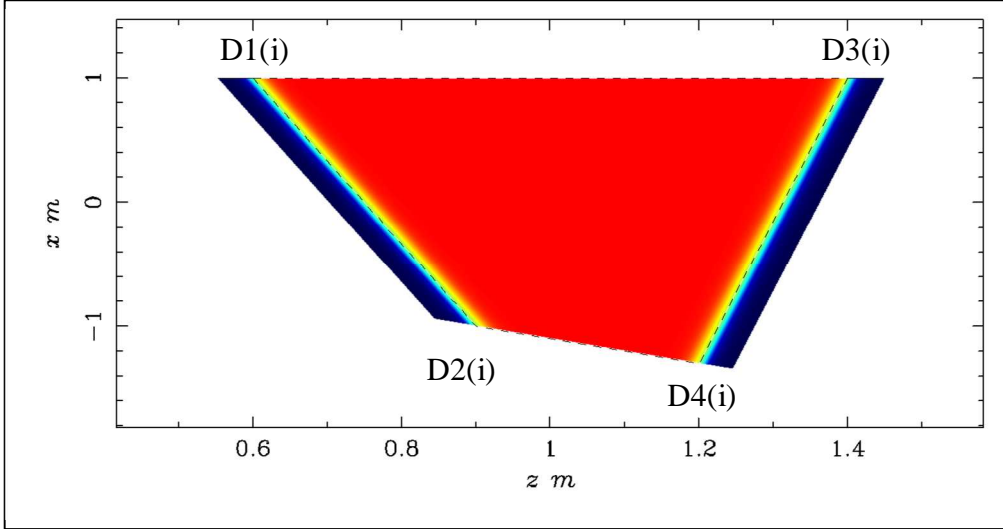
Fig. 4 Example for the definition of a dipole: The entrance and exit face of the dipole are defined by the lines D1(i) = (1.0, 0.6) to D2(i) = (-1.0, 0.9) and D3(i) = (1.0, 1.4) to D4(i) = (-1.3, 1.2) . The lines D1 - D2 and D3 - D4 are associated with the taper parameters D\_Gap(1,i) and D\_Gap(2,i) . The entrance and exit lines form together with the extrapolated connecting lines D1 - D3 and D2 - D4 the area in which the dipole field is defined. Note the order of the corner points. Exchanging D3 and D4 would be no valid input.
