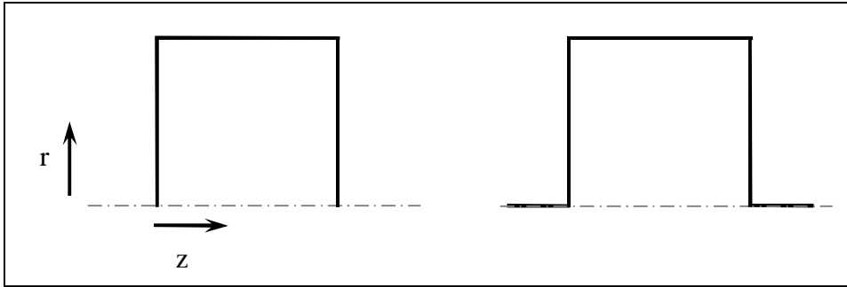
Fig. 1 Sketch of closed apertures. The aperture on the left does not ensure that particles are lost with the condition r > r_{\max} since the closing walls have zero wall thickness.
