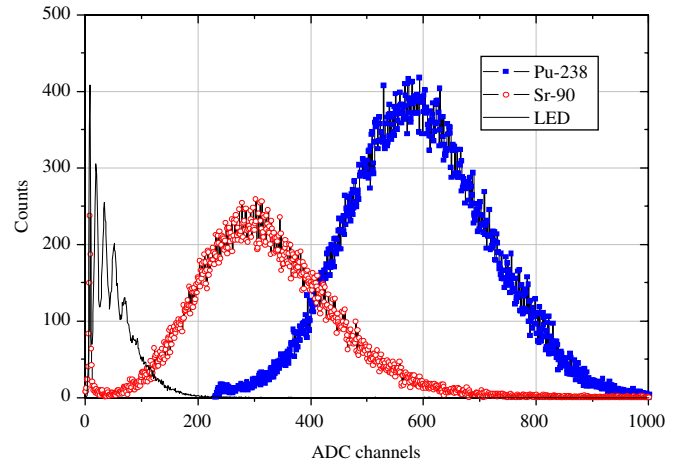
Fig. 7. SiPM spectra for LED, \beta -particles from \text{Sr}^{90} and \alpha -particles from \text{Pu}^{238} source.
