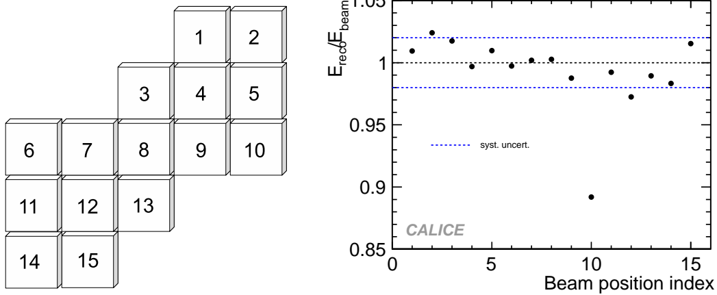
Figure 17. Schematic view of tile positions in an AHCAL scintillator plane used for the uniformity test (left) and uniformity of the calorimeter response for various positions of incident beam with respect to the detector (right). Tile position eight is approximately in the center of each calorimeter layer. The dashed lines show the systematic uncertainties. Statistical errors are negligible.
