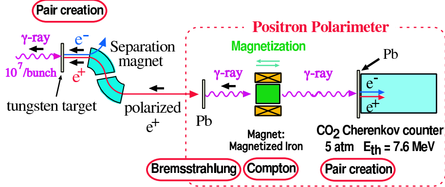
FIG. 4: Schematic drawing for the e^+ production apparatus and the polarimeter. Polarized \gamma -rays are incident on a 1mm thick tungsten plate resulting in electron-positron pair creation. The separation magnet installed after the tungsten plate efficiently extracts high energy positrons, which generates circularly polarized \gamma -rays through bremsstrahlung in the lead. The transmission of the \gamma -rays can be measured with the \text{CO}_2 -gas Cherenkov counter.
