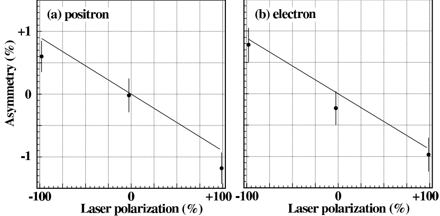
FIG. 6: Measured asymmetry as a function of the circular polarization of a laser beam. Straight lines are result of linear fitting with a constraint of passing the origin (0,0); (a) result of the positron measurement, (b) result of the electron measurement. Note: When the direction of photon spin and the direction of it's momentum is paralell, we call it right-handed. When a laser beam is 100% right-handed polarized, we call it +100%.
