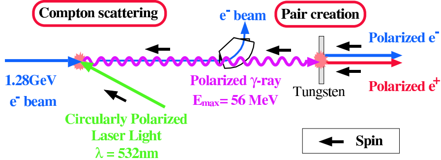
FIG. 1: A fundamental scheme of polarized e^+ production. Right-handed polarized laser photons are backscattered off relativistic electrons resulting in production of left-handed polarized \gamma -rays in the forward direction (in the high energy part of the spectrum). Pair creation of the \gamma -rays through a tungsten plate generates left-handed positrons in the high energy part.
