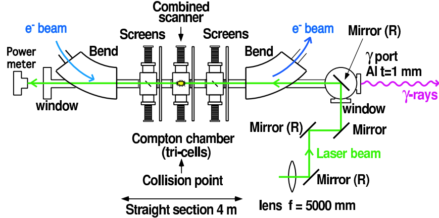
FIG. 3: Experimental setup of the polarized \gamma -ray production system including the Compton chamber with three cells, the laser optics with three remotely controllable mirrors, and electron beam line. Laser-electron collisions take place at the central cell of the Compton chamber.
