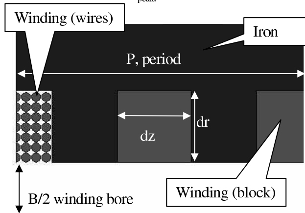
Figure 1: Diagram showing the 2d planar undulator models, the innermost winding has a high mesh density to model the peak field in individual wires accurately
