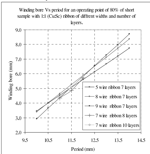
Figure 3: Some 2d results for the different configurations. The results are normalised for an operating point 80% of short sample.
