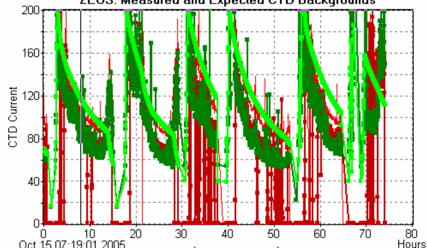
ZEUS: Measured and Expected CTD Backgrounds
