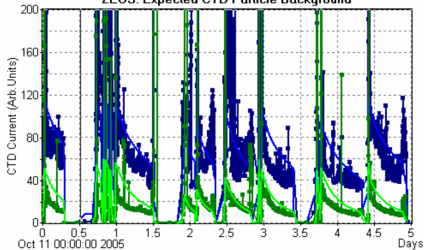
ZEUS: Measured and Expected CTD Backgrounds
