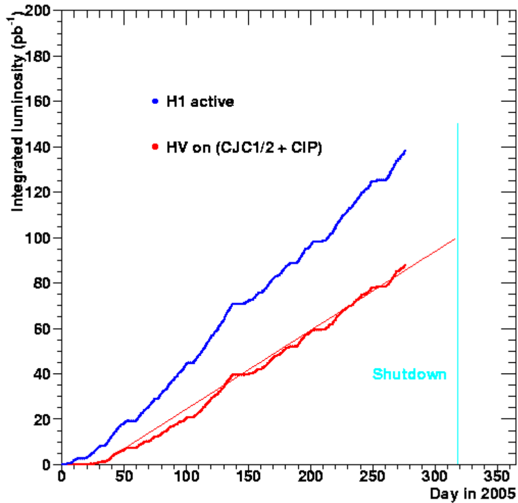
H1 Luminosity 2005
