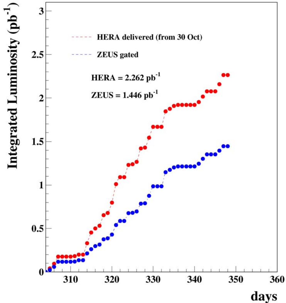
HERA/ZEUS luminosity
